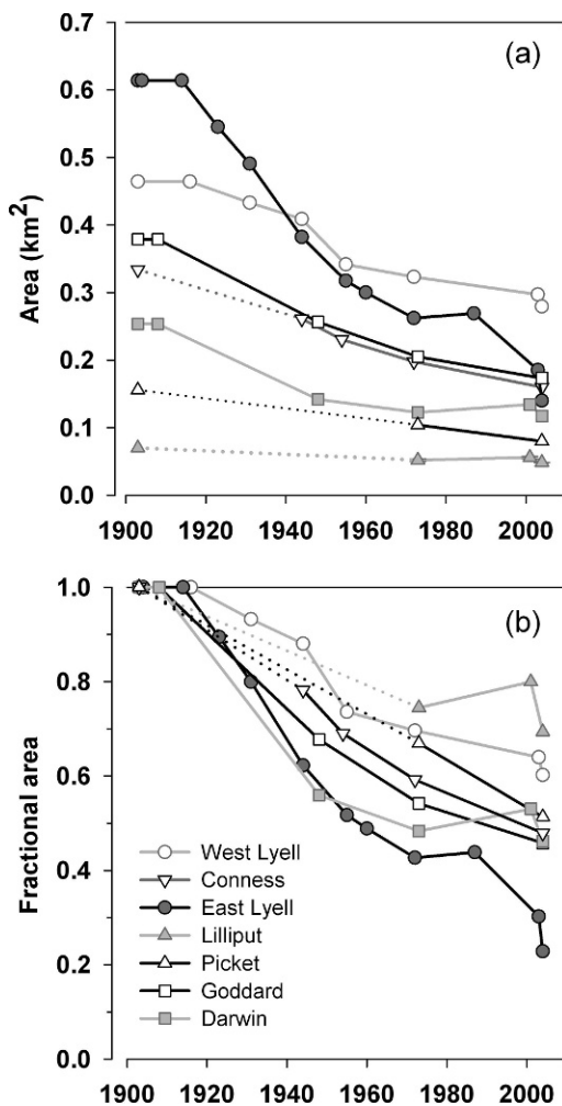
FIGURE 4. (a) Surface area and (b) fractional area changes at the seven glaciers in the Sierra Nevada over the past century (1903–2004). Dotted lines represent assumed change for glaciers lacking early 1900s photographic evidence. Error bars are omitted as error is smaller than symbol.
