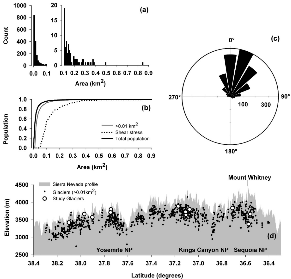
FIGURE 2. Characteristics of the population of glaciers and perennial snowfields in the Sierra Nevada, California: (a) population as a function of area ( \text{km}^2 ), note change in y-axis for glaciers >0.01 \text{ km}^2 ; (b) cumulative sum with area for the total population, for glaciers >0.01 \text{ km}^2 , and for the population of features with an estimated basal shear stress >10^5 \text{ Pa} ; (c) total population as a function of aspect, using 20^\circ bins; and (d) the north-to-south distribution of the glacier population >0.01 \text{ km}^2 (black dots) and study glaciers (white circles) overlaid on elevation of the Sierra Nevada (gray).
