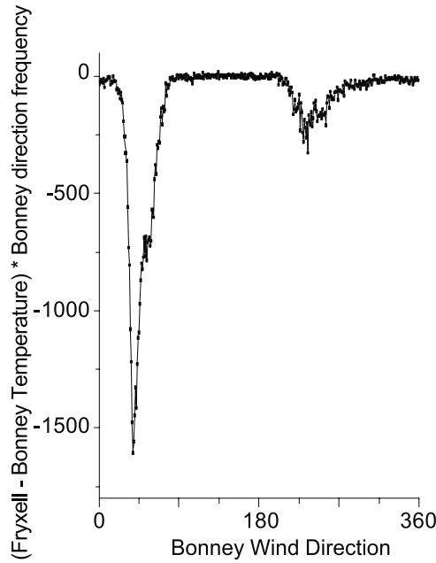
Figure 14. Plot of the difference between Fryxell and Bonney summer temperature weighted by Lake Bonney wind direction frequency versus wind direction at Lake Bonney (in 1^\circ increments).
