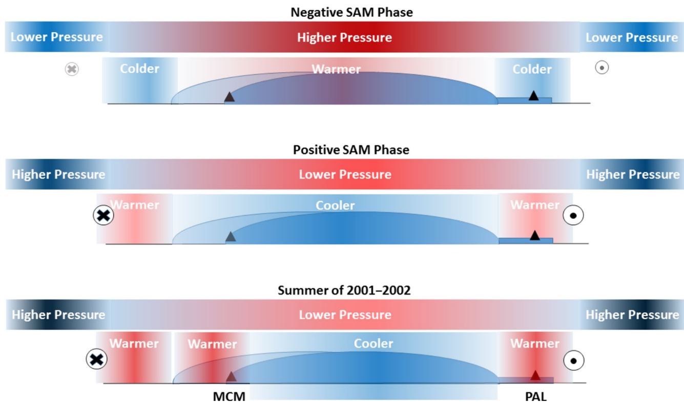
Figure 4. A conceptual diagram of the negative and positive phases of the Southern Annular Mode over Antarctica and its effect on surface air temperatures and pressure. The circum-Antarctic wind flow direction and velocity are shown by the arrow out of the page (dot and circle) and the arrow into the page (x and circle). The larger bold markings indicate faster winds. The solid triangles represent the locations of MCM (left) and PAL (right). The double edge of the Antarctic continent on the left represents the geographical position of MCM within the Ross Sea away from the outer edge of Antarctica. The warmer air temperatures at MCM during the summer of 2001–2002 were due to local effects in response to hemispheric conditions.
