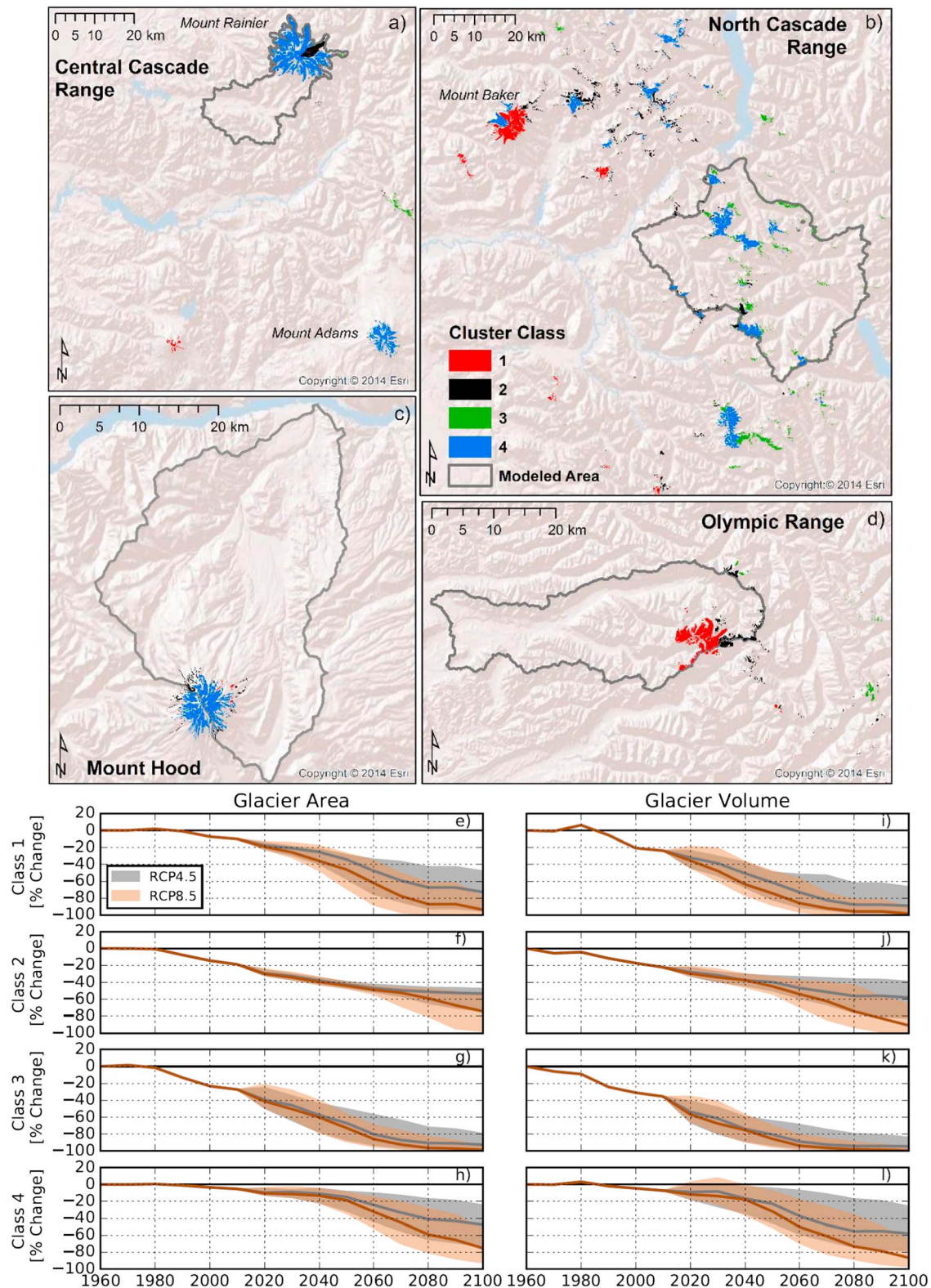
Figure 11. (a–d) Classification of PNW glaciers using K-means cluster analysis based on each glacier’s local climatology defined by Parameter elevation Regression on Independent Slopes Model (PRISM). Glacier polygons were defined by Fountain et al. (2017). (e–h) Modeled historical and future projections of glacier area and (i–l) volume change for each aggregated cluster classification. The range is defined by the minimum and maximum amounts of projected losses in glacier area for the period 1960–2099 in modeled projections for the glaciers in the study basins. This range represents a 10-member ensemble of projections for each emission pathway scenario (Representative Concentration Pathway [RCP4.5] and RCP8.5). The historical simulation and the ensemble median is shown with the solid lines.
