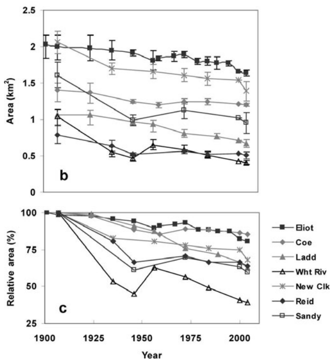
Fig. 3. Change on seven of Mount Hood's glaciers over the 20th century: (a) map of areal change, 1907–2004; (b) area change with time for individual glaciers; and (c) fractional area change.
