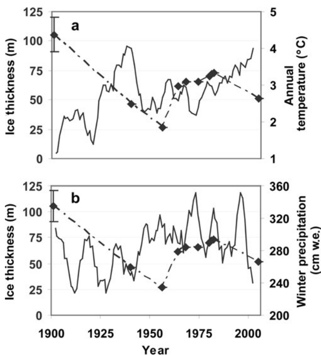
Fig. 4. Ice thickness at the B profile (dashed line) plotted with a 5 year running average annual temperature (a) and winter precipitation (b) (Daly and others, 1997).
