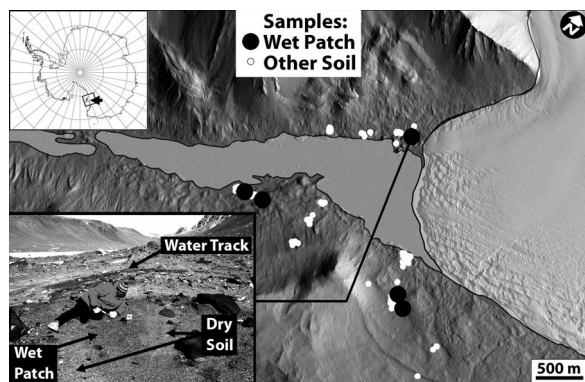
Figure 1. Sampling sites in the Lake Hoare Basin, Taylor Valley, Antarctica (some sites yielded multiple soil samples from multiple wet patches). Glacier, lake, and soil contacts are highlighted. Inset map shows the general location of Southern Victoria Land, Antarctica (box) and the location of the MDV (arrow). Inset sampling example shows a wet patch with a water track \sim 10 m behind it, and separated by a topographic divide.
