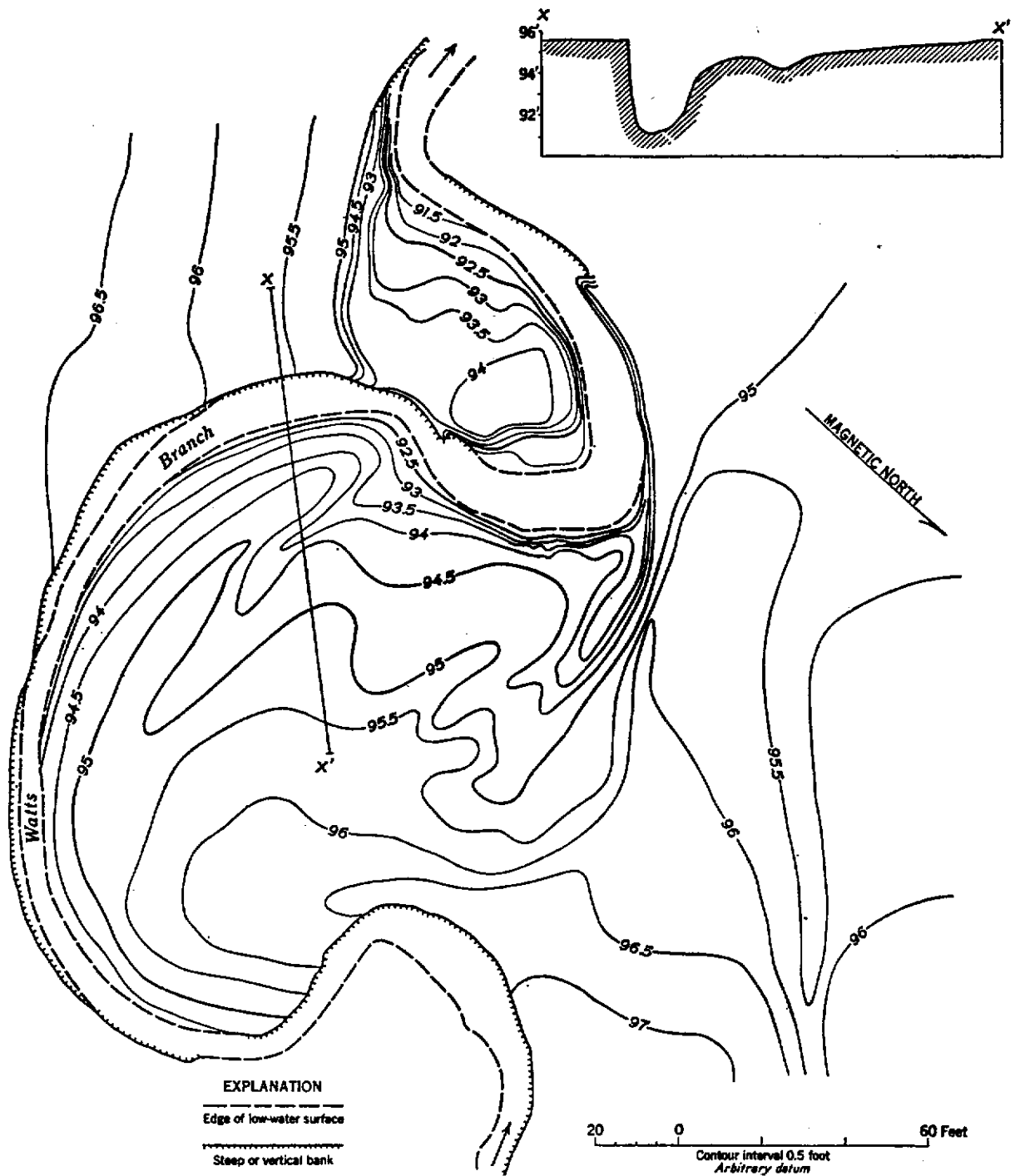
FIGURE 7.—MAP AND CROSS SECTION OF A TYPICAL POINT BAR OF THE FLOOD PLAIN OF WATTS BRANCH, 1 MILE NORTHWEST OF ROCKVILLE, MARYLAND After Wolman and Leopold (1957)
