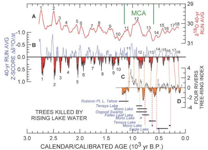
Fig. 27. Comparison of Pyramid Lake \delta^{18}\text{O} record (panel A) and its derivative with respect to time (panel B) with a northern Sierra Nevada tree-ring record (panel C) and ages of tree stumps killed by rising lake waters (panel D). (A) 40-yr running average of \delta^{18}\text{O} record from PLC97-1. Oscillations in \delta^{18}\text{O} are numbered 1–18. (B) Smoothed derivative of normalized \delta^{18}\text{O} record shown in panel A; positive values of the derivative, shown as solid areas below the zero line, indicate times when the lake was falling. Hydrologic droughts have been numbered 1 through 18. MCA refers to the time interval occupied by the Medieval Climatic Anomaly (1150–600 cal yr BP). C. Northern Sierra Nevada tree-ring record (Meko et al., 1999); solid areas indicate drought periods. D. Ages of tree stumps killed by rising lake waters (Lawrence and Lawrence, 1961, Stine 1990, 1994). Data for tree stumps at Rubicon Point ( 1240 \pm 40 ^{14}\text{C} yr BP, Beta 133581) and Fallen Leaf Lake ( 850 \pm 40 ^{14}\text{C} yr BP, Beta 133580) are part of this study. Solid blue dots indicate best estimates of drought termination. Horizontal black lines reflect uncertainty in the calendar-age estimates of drought termination. Solid orange lines indicate possible correlation between core-based and tree-ring-based drought records. Dashed red lines indicate tree-ring-based timing of drought terminations.
