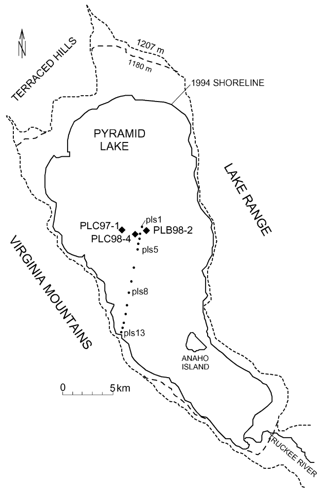
Fig. 10. Coring sites, Pyramid Lake, Nevada. Water depths are >100 m at the sites of the piston and box cores (PLC97-1, PLC98-4, PLB98-2). PLS samples are sediment-water interface samples taken along a transect starting in the deep basin of Pyramid Lake and ending at Pelican Point. The inner dashed line indicates the area that Pyramid Lake achieved during overflow to the Winnemucca Lake basin.
